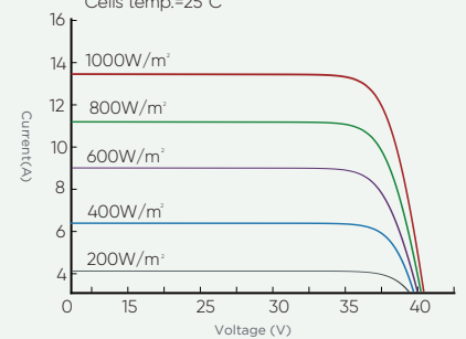
Current-Voltage Curve
